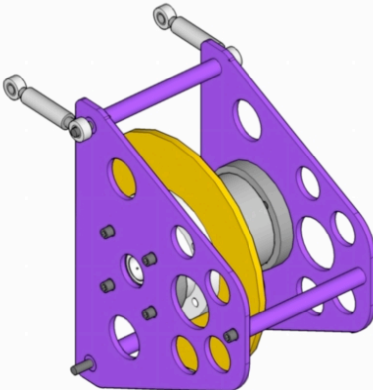
Ford Sierra Based Limited Slip Chain Drive Differential (Typical Installation)
